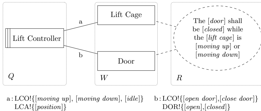
Figure 2: A problem diagram describing door behaviour
