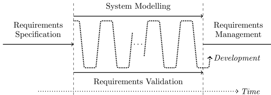
Figure 10: The Iterative Requirements Development Process
