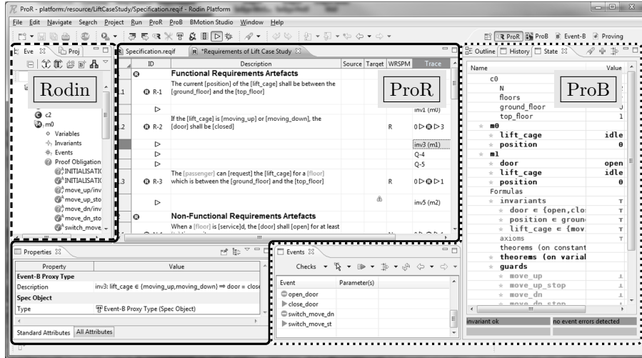
Figure 12: Integration of ProR with Rodin and ProB
