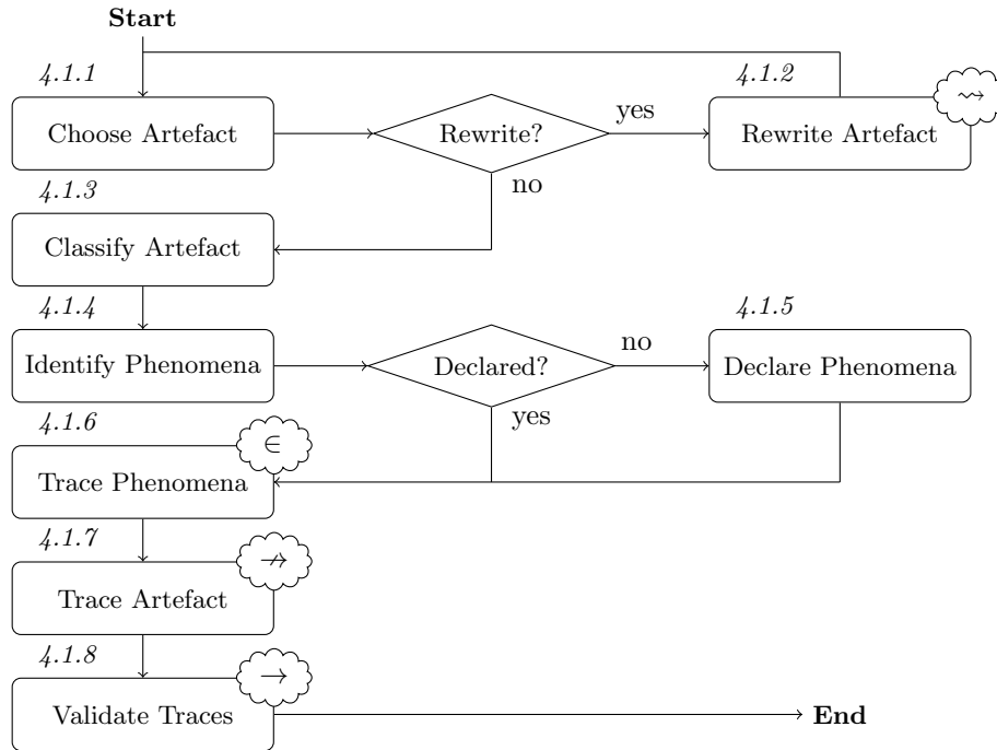
Figure 11: The Requirements Modelling and Validation Process
